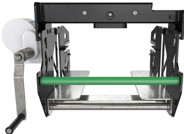
Svendborg Brakes' LBS Yaw Brake Lifting tool allows service teams to carry out wind turbine maintenance in-situ.
